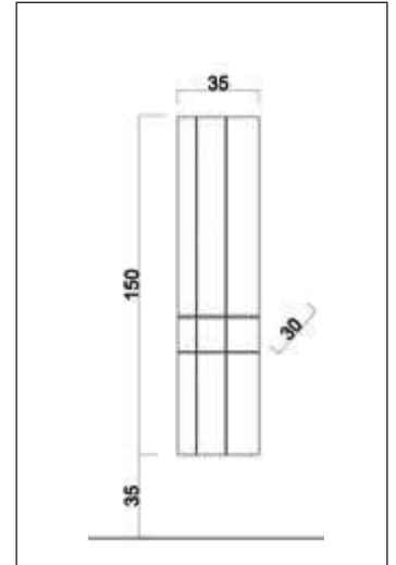
TALL CABINET | BOY DOLABI
