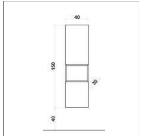
TALL CABINET | BOY DOLABI
