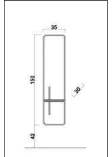
TALL CABINET | BOY DOLABI
